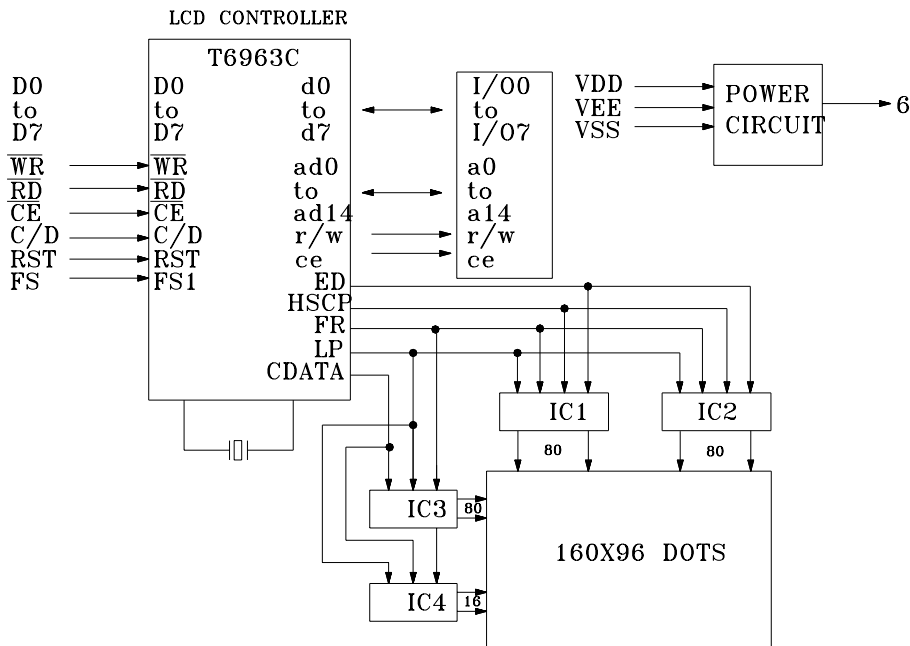
BLOCK DIAGRAM
